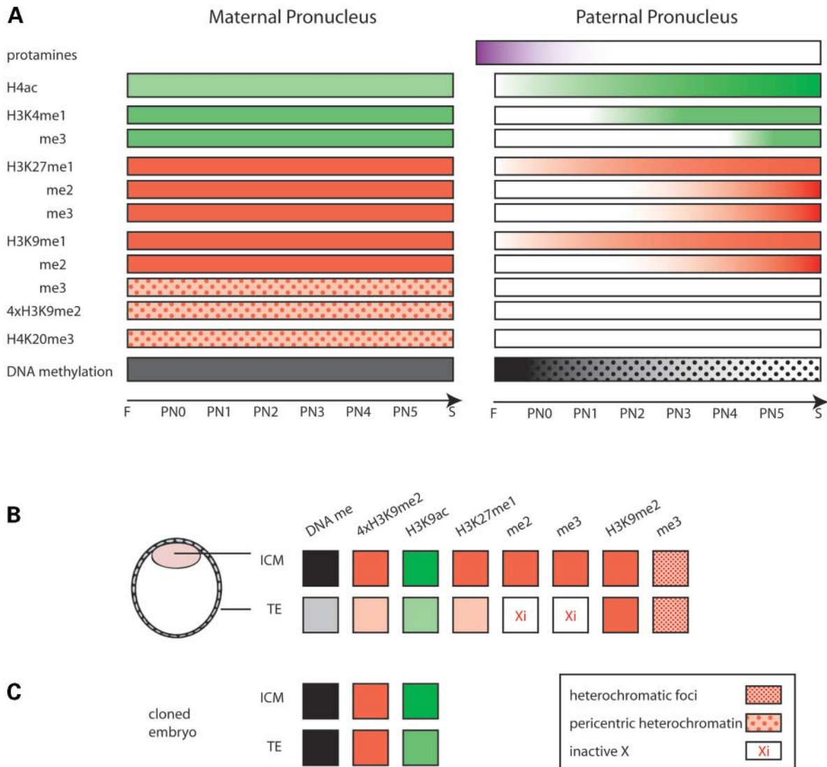
Figure 2. Preimplantation epigenetic reprogramming and cloning. (A) Remodelling in the mouse maternal and paternal pronuclei. Transcriptionally permissive modifications (green) and repressive modifications (red) are shown with shading intensity indicative of level of modification from fertilization (F) through pronuclear stages (PN0–PN5) (14) and syngamy (S). In the paternal pronucleus: protamines (purple) are exchanged for histones which are hyperacetylated (14,15), and carry H3K27me1 and H3K9me1 (42), but initially lack H3K4me1 and me3 (37), H3K27me2* and me3 (38), H3K9me2 (36) and me3*, heterochromatic histone methylation (4 × H3K9me2 antibody) (34,35) and H4K20me3 (39); DNA methylation (black) is lost actively before DNA replication at PN3–PN4, except at pericentric heterochromatin, some repeats (IAPs) and paternally methylated imprints (14–17,20,21); H3K4me1 and me3 (37), H3K27me2*, me3* and H3K9me2 (36) accumulate during pronuclear development. H3K9me2 and me3*, heterochromatic histone methylation and H4K20me3 particularly mark pericentric heterochromatin in the maternal pronucleus (34–36,39). (B) Epigenetic differences between the ICM and trophectoderm. De novo methylation results in a methylated ICM, but less methylated TE in mouse (15,17); bovine (26,54); sheep (18). H3K9ac and heterochromatic histone methylation are re-established in the blastocyst preferentially in the ICM compared to the TE (54). H3K27me1, me2* and me3 are present predominantly in the ICM, and H3K27me2* and me3 only mark the inactive X chromosome in the TE (in the mouse) (38). H3K9me2 stains evenly between ICM and TE and across the genome (38). H3K9me3 marks heterochromatic foci in the ICM and TE (38). (C) In cloned embryos, DNA methylation (bovine and sheep), heterochromatic histone methylation (bovine) and H3K9ac (bovine) remain at abnormally high levels in the TE (17,18,26,54). Asterisk marks refer to data not shown (38).
